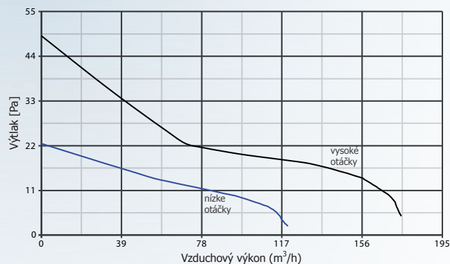
ME 120/5"
