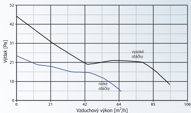
ME 100/4"
